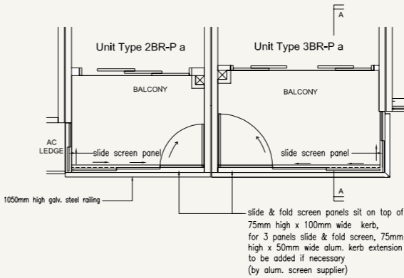
TYPICAL PLAN OF BALCONY WITH SCREEN
